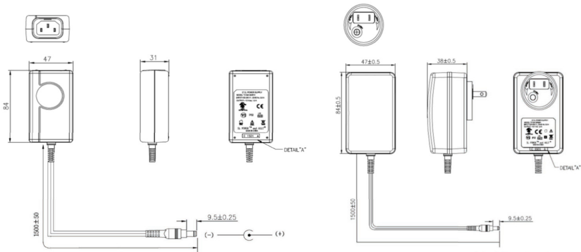
IEC60320 C14 Receptacle, 2.5 x 5.5 x 9.5 mm Barrel Connector
