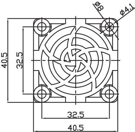
LOWER HOUSING
