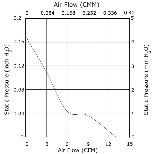
CFM-5015V-247-290
