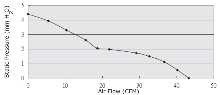
CFM-8025B-235-364
