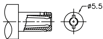
MATING PLUG
