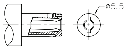
MATING PLUG Jack Insertion Depth: 7.3 mm
