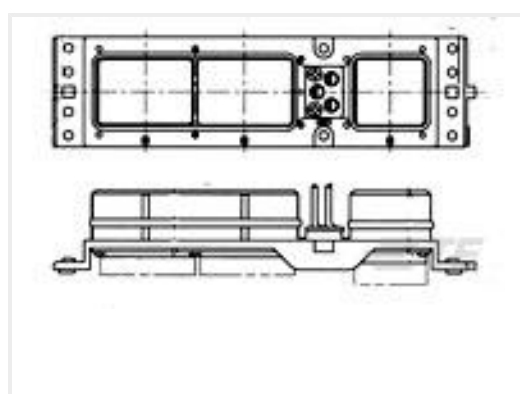
TE Part #1663557-1 PLUG ASSY, SZ 2, ARINC 600
