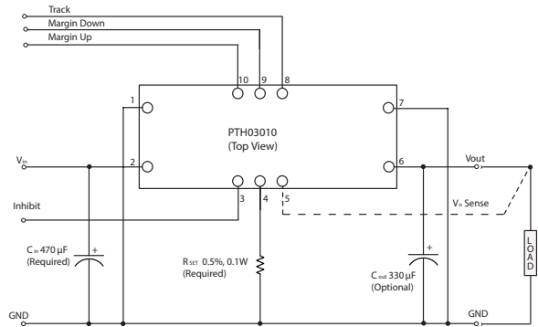
Figure 4 - Standard Application
