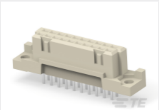
TE Part #254370-E STVB/3 20 F AB VV 7-00 TL 4,0 * 247 E007
