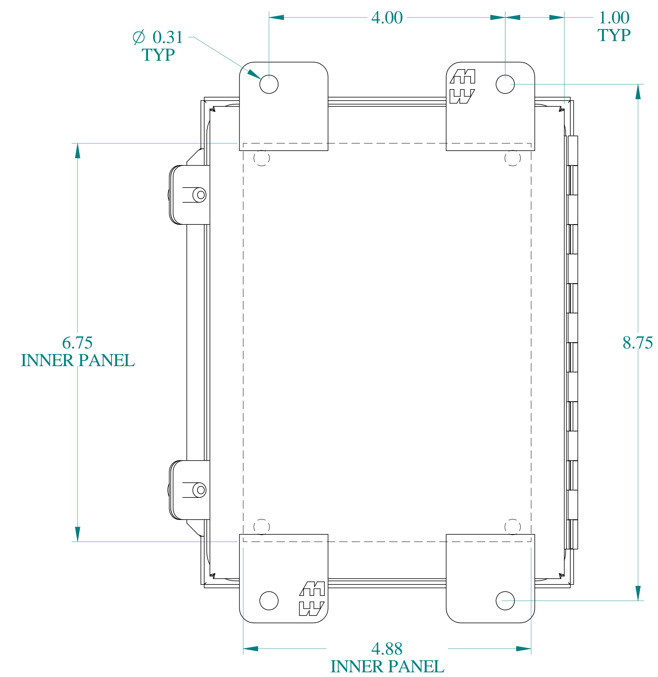
BACK VIEW
