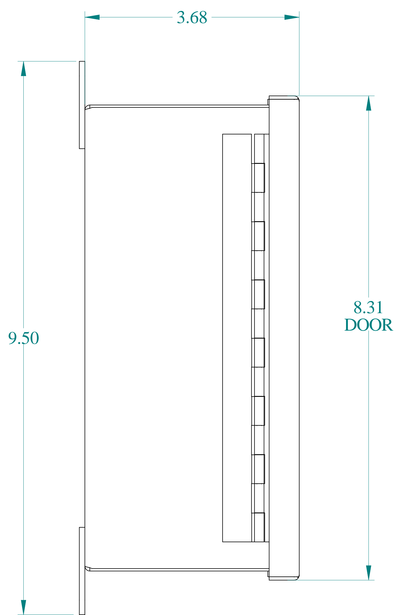
SIDE VIEW
