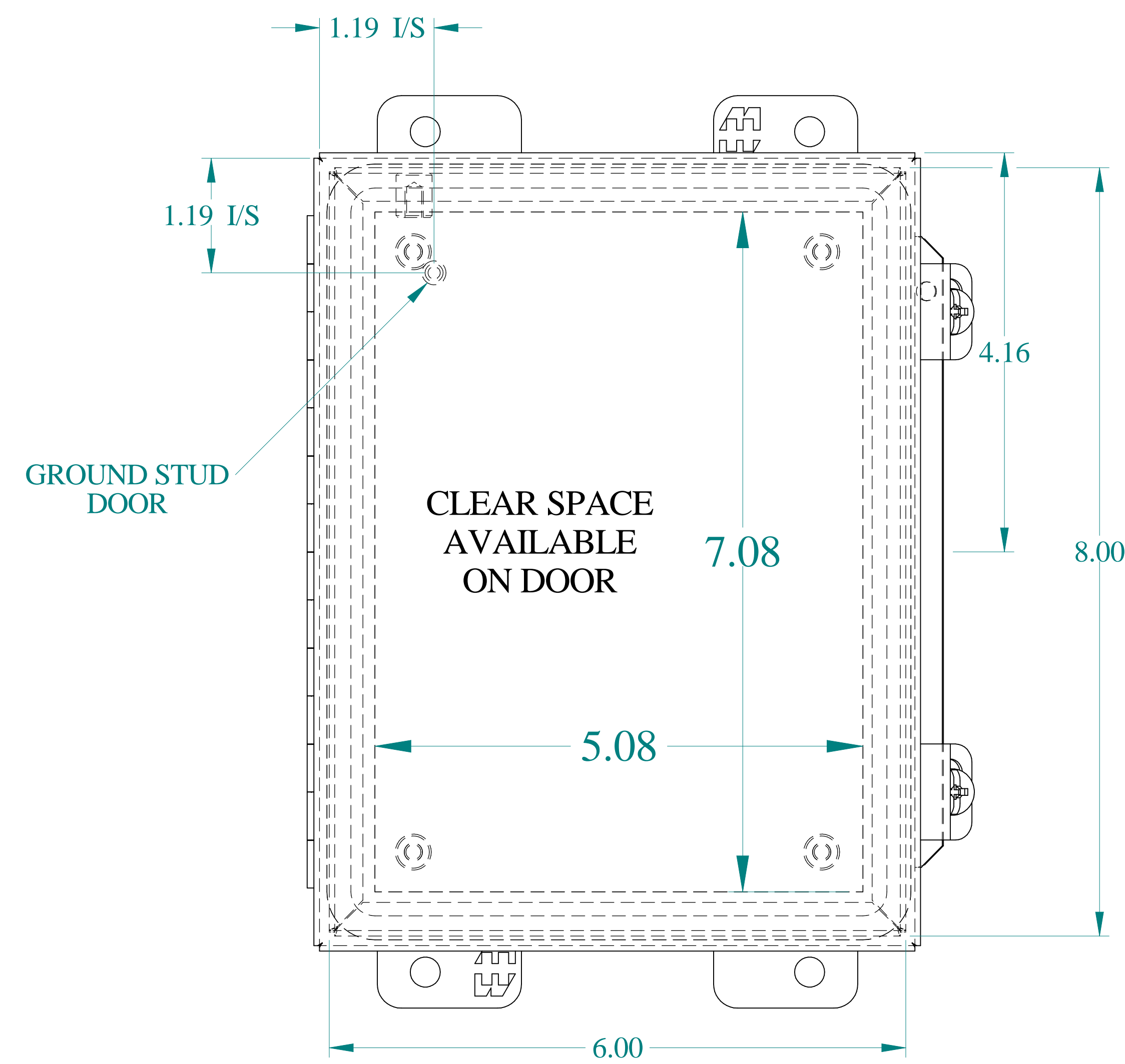
FRONT VIEW
