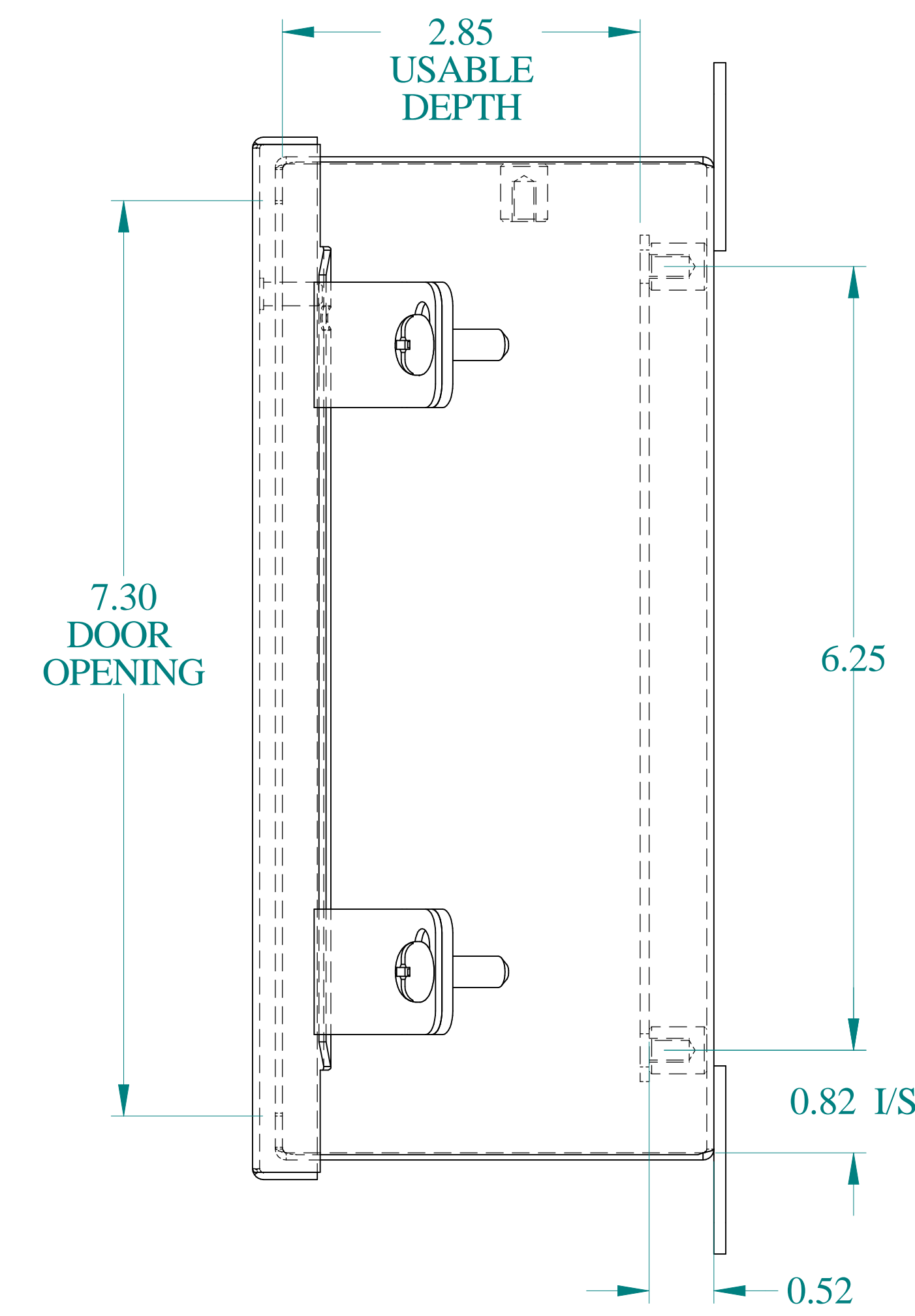
SIDE VIEW
