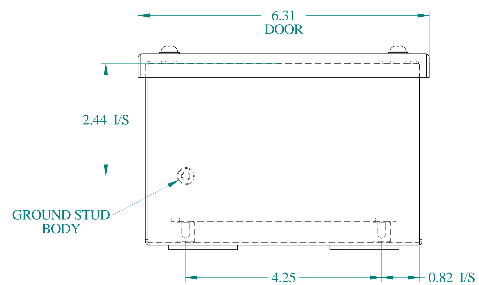
BOTTOM VIEW
