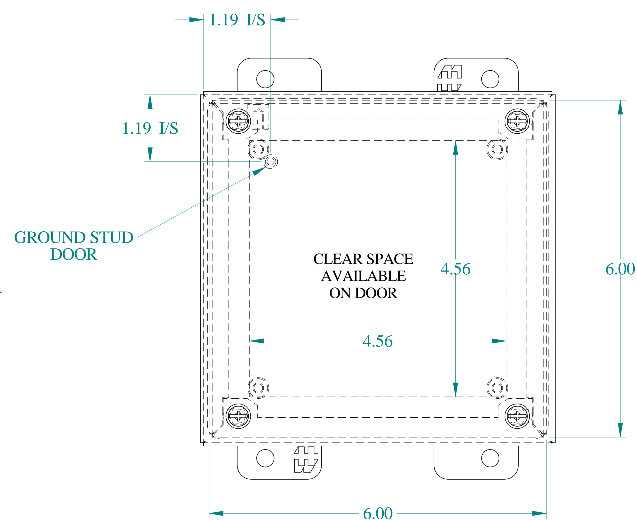
FRONT VIEW
