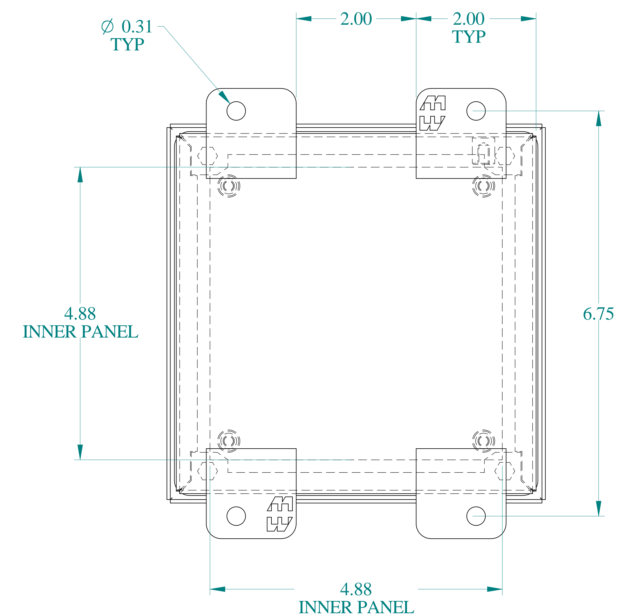
BACK VIEW
