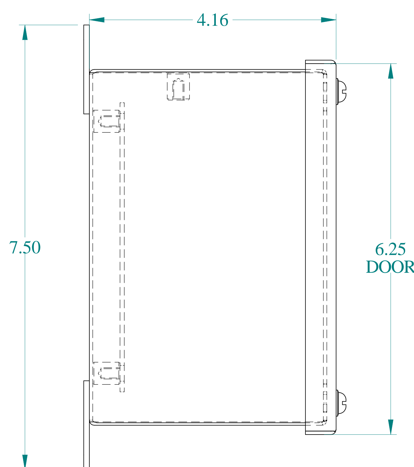
SIDE VIEW
