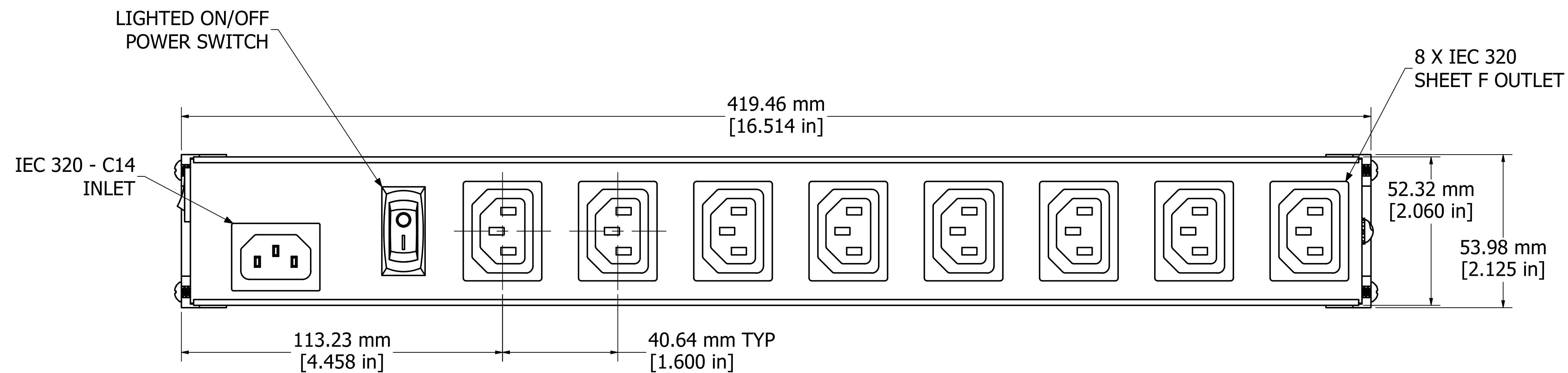
ASSEMBLY - VIEW FROM TOP
