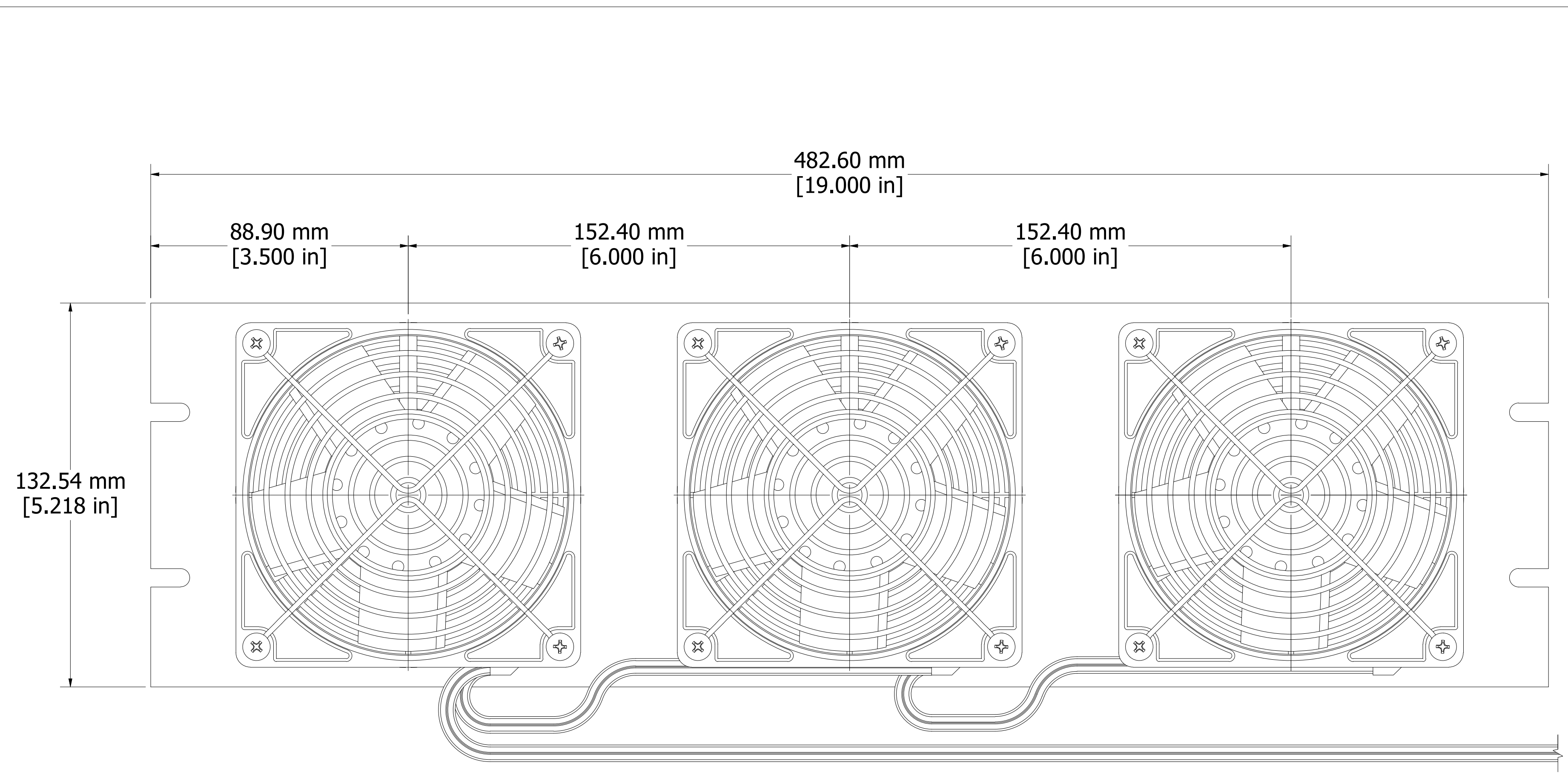
ASSEMBLY - VIEW FROM REAR
