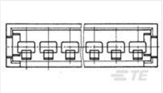
TE Part #280631 AMPMODU II COSI PIN HSG, SGL ROW, 8 POS.
