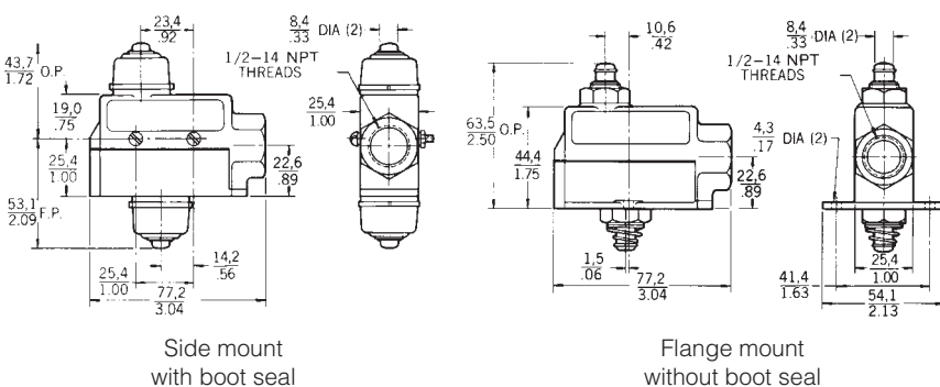
Figure 11. Top pin plunger reset switch
