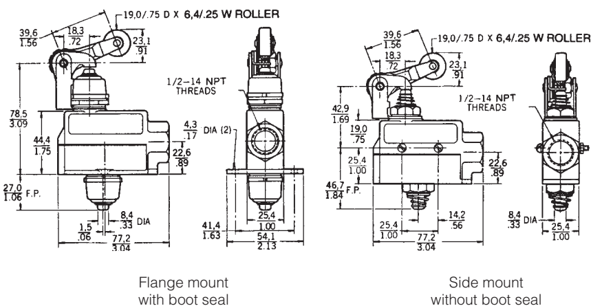
Figure 10. Top roller plunger reset switch
