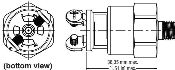
Figure 12. Screw terminal
