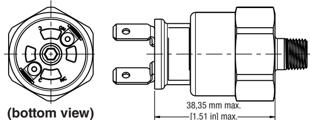
Figure 11. Blade terminal
