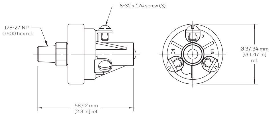
Figure 29. 5000 Series Dimensions
