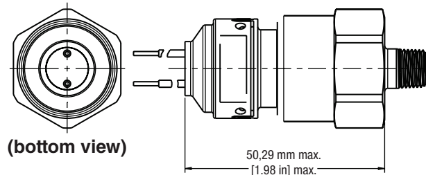
Figure 10. Wire out
