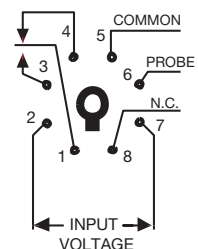
PIN CONFIGURATION
