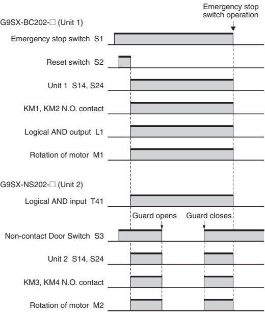
Timing chart
