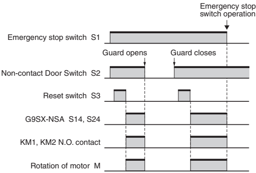
Timing chart
