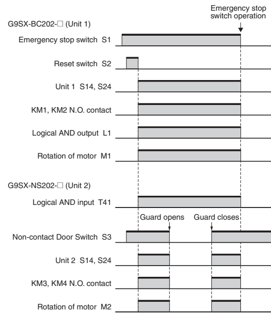
Timing chart
