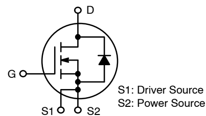
N-CHANNEL MOSFET
