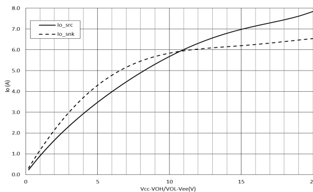
Figure 19. Output Current vs. Output Voltage Drop
