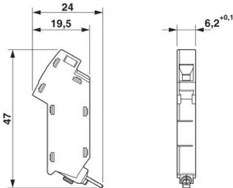
Dimensional drawing
