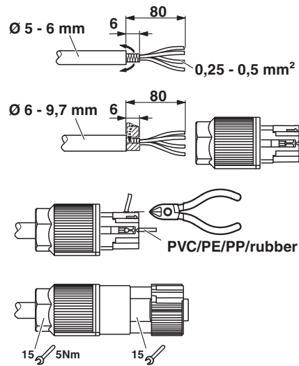
Dimensional drawing
