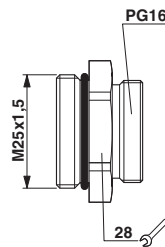
Dimensional drawing
