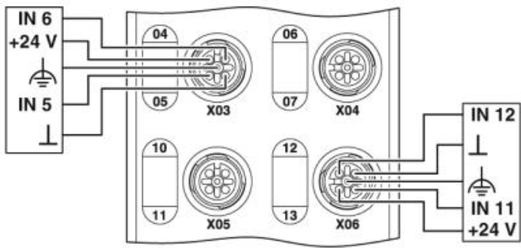
Connection diagram
