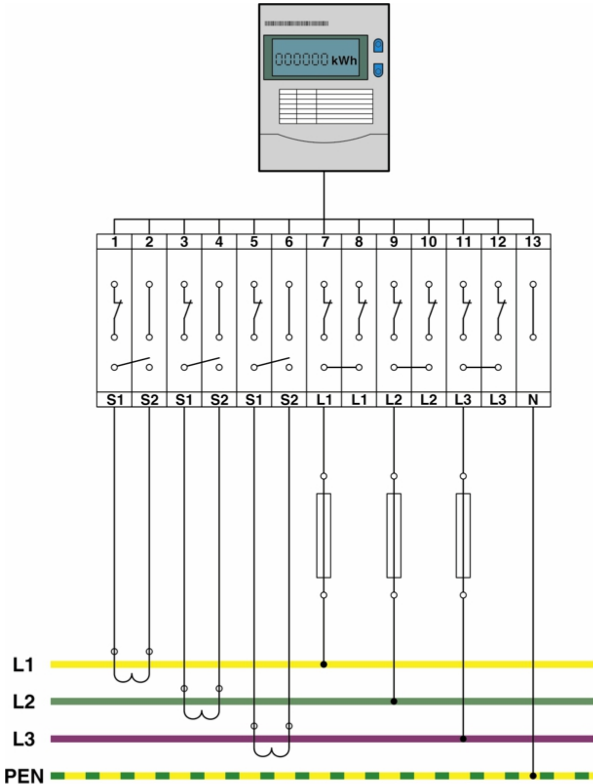
Circuit diagram
