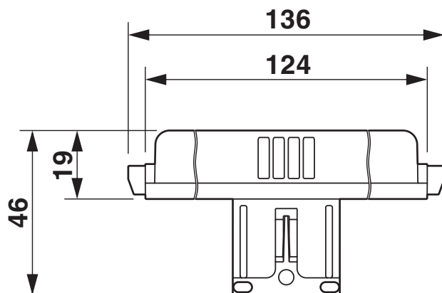
Dimensional drawing
