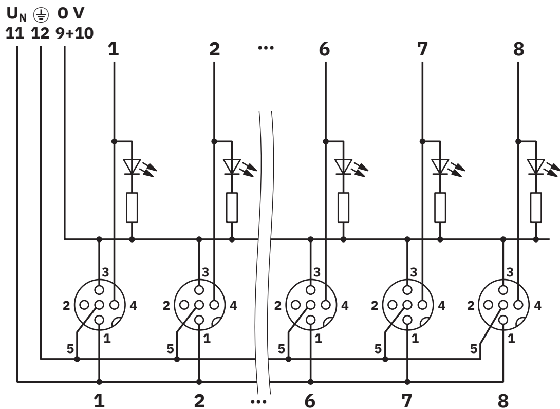
Circuit diagram
