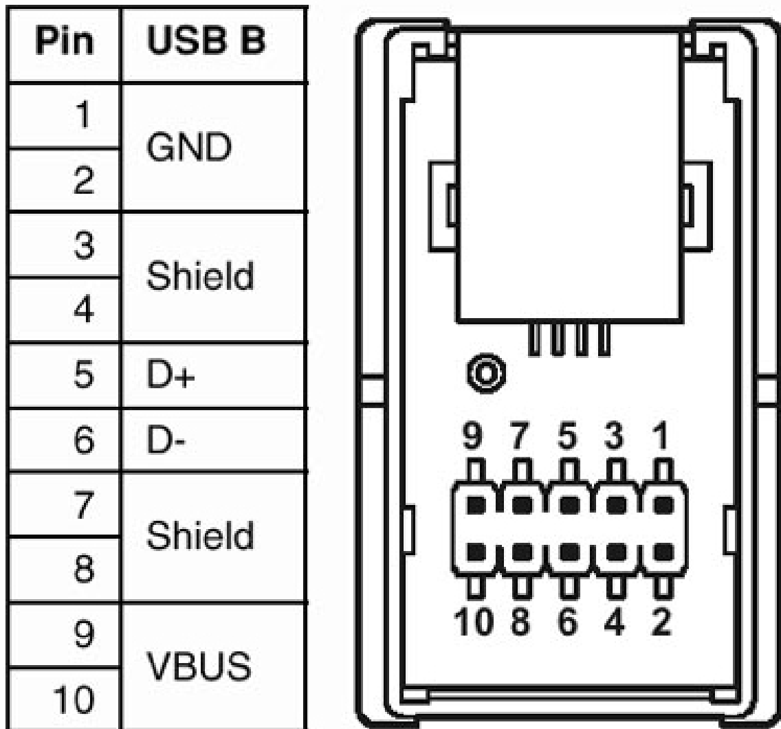
Contact assignment
