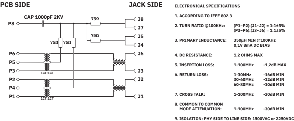
Circuit diagram
