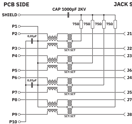
Circuit diagram JACK SIDE
