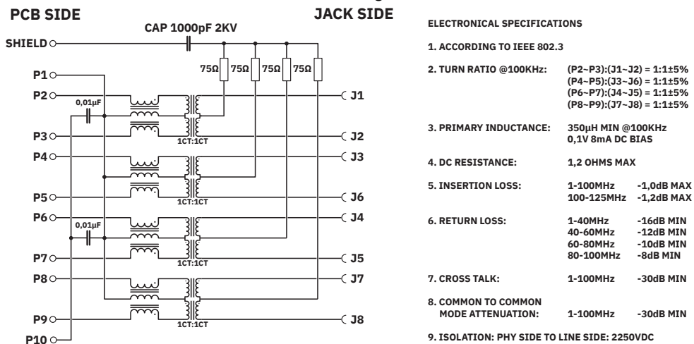
Circuit diagram
