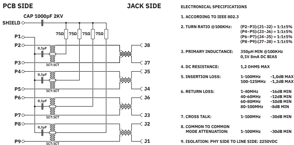
Circuit diagram
