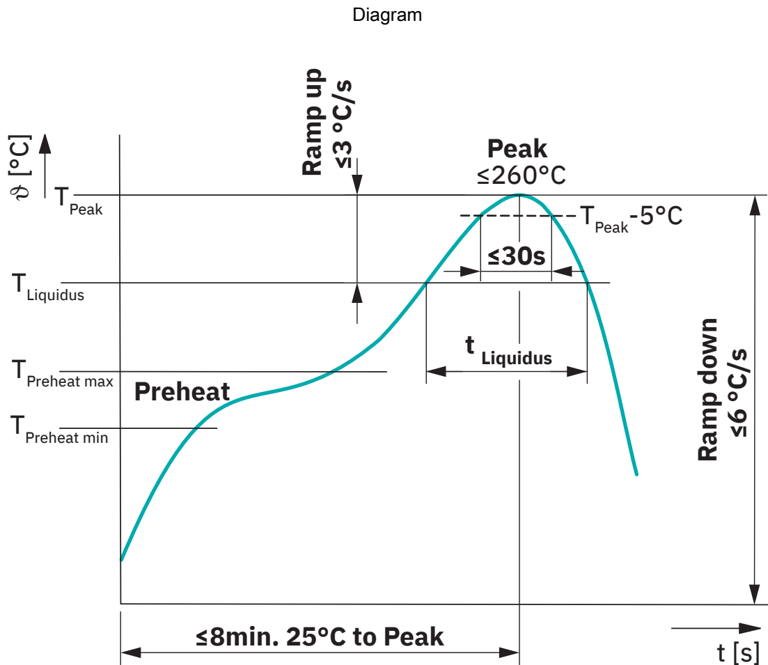
Classification reflow soldering profile
