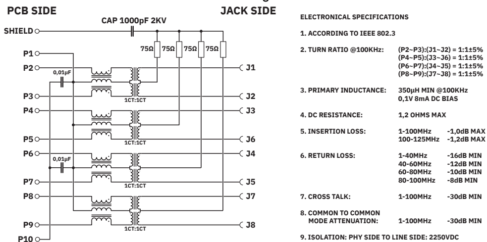
Circuit diagram JACK SIDE
