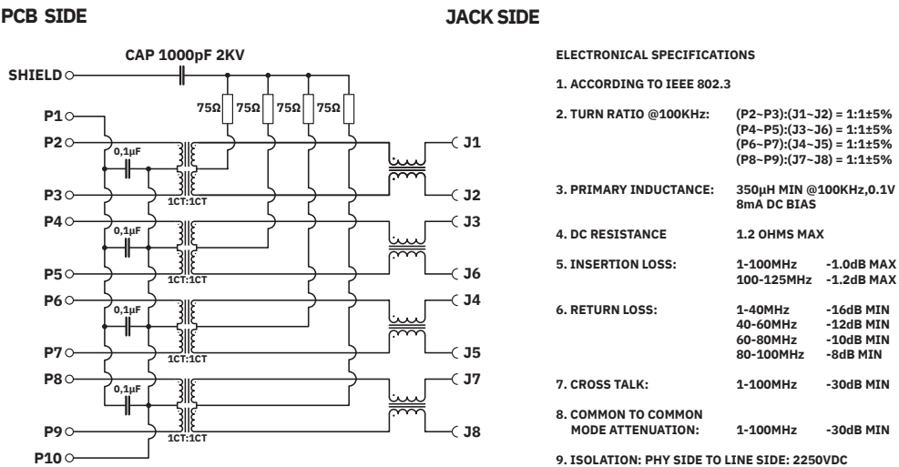
Circuit diagram
