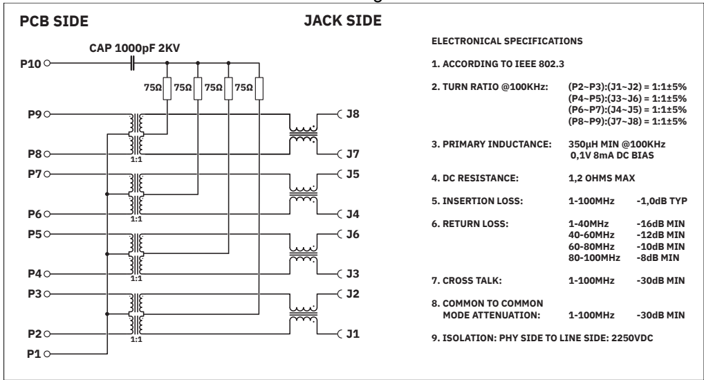
Circuit diagram
