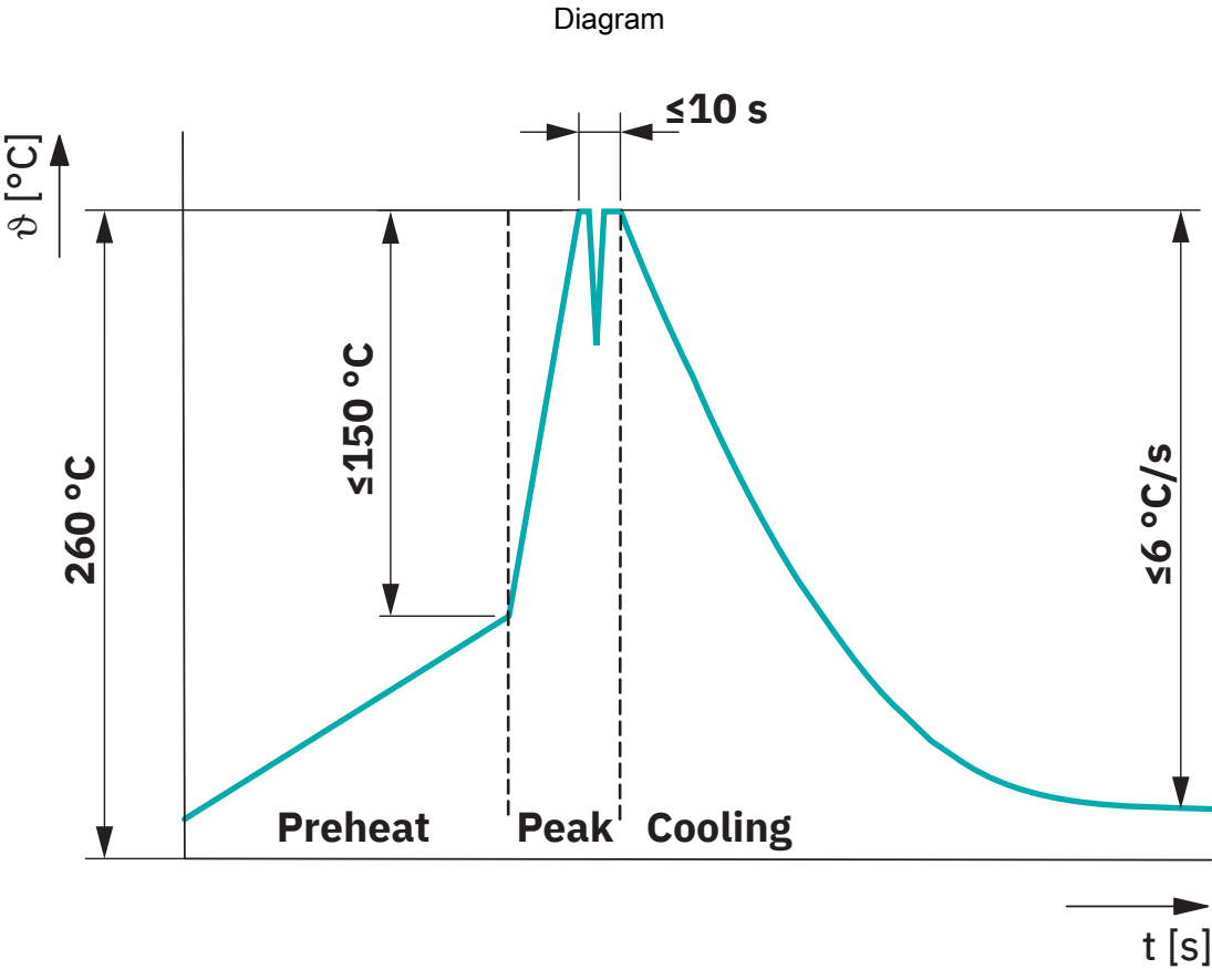
Classification wave soldering profile
