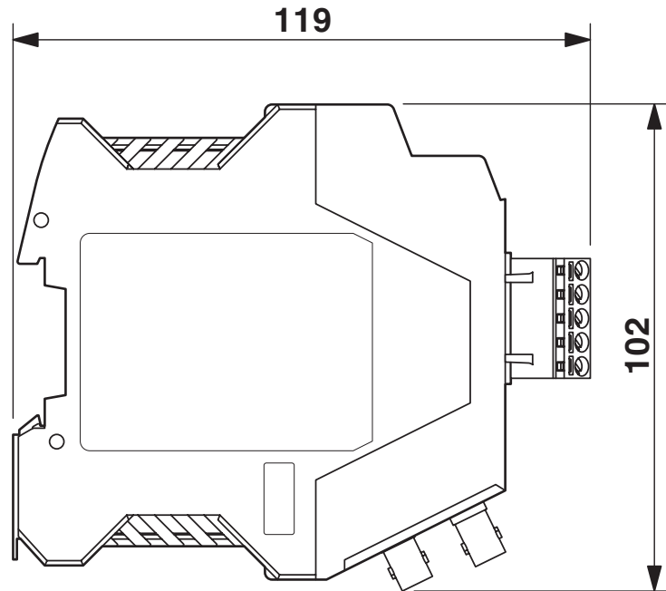
Dimensional drawing
