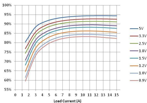
Figure 5. Efficiency vs. Load. V_{in} = 12 V, F_{sw} = 500 kHz
