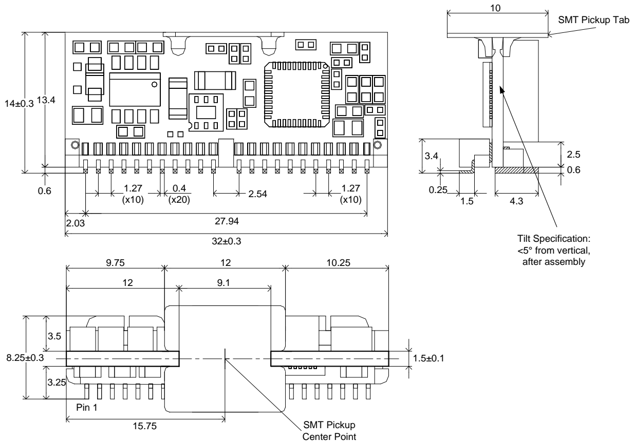
Figure 58 Mechanical Drawing
