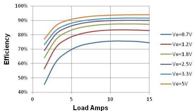
Figure 6. Efficiency vs. Load. V_{in} = 12 V, F_{sw} = 1 MHz
