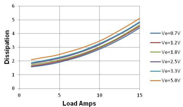
Figure 12 Dissipation vs Voltage. V_{in}=12V , F_{sw}=1MHz
