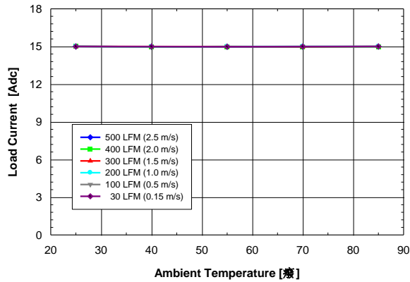
Figure 3. Available output current vs. ambient air temperature and airflow rates for converter DP7115G mounted horizontally with air flowing from input to output, MOSFET temperature 120 °C, V_{in} = 12 V, V_{out} = 5 V, and F_{sw} = 500 KHz
