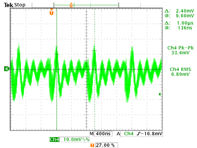
Figure 46. Input Voltage Noise with Interleave
