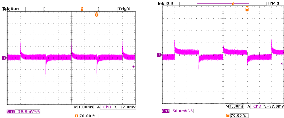
Figure 50. Transient Response with Regulation set to 0.0 mV/A. Figure 51. Transient Response with Regulation set to 3.72 mV/A
