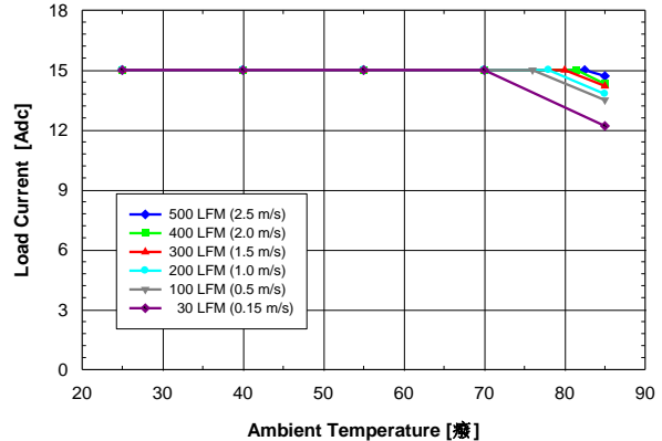
Figure 4. Available output current vs. ambient air temperature and airflow rates for converter DP7115G mounted horizontally with air flowing from input to output, MOSFET temperature 120 °C, V_{in} = 12 V, V_{out} = 5 V, and F_{sw} = 1 MHz
