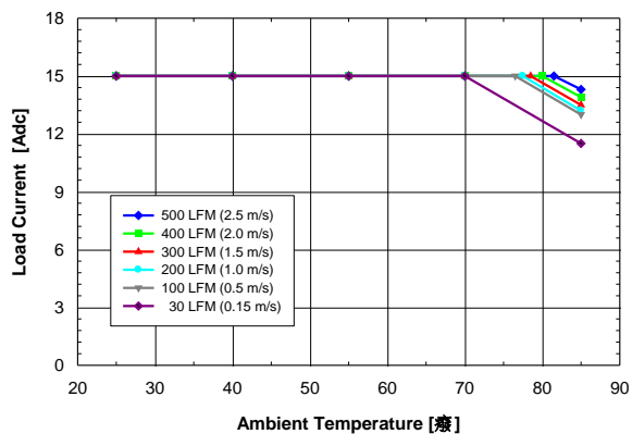
Figure 3. Available output current vs. ambient air temperature and airflow rates for converter DP7115G mounted horizontally with air flowing from input to output, MOSFET temperature 120 °C, V_{in} = 12 V, V_{out} = 5 V, and F_{sw} = 500 KHz
