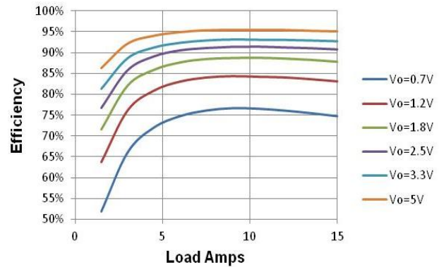
Figure 8 Efficiency vs Load. V_{in}=8V , F_{sw}=1MHz
