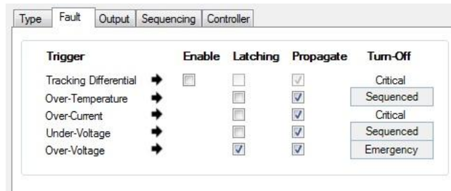
Figure 33. GUI dPOL Fault Propagation Option Window
