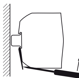
Fig. 15b Dismounting from DIN-rail. Use proper tool (min. 3 mm screwdriver) and adequate force.
