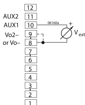
Adjustment with V_{ext}
