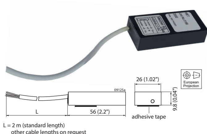
Fig. 25 Temperature sensor
