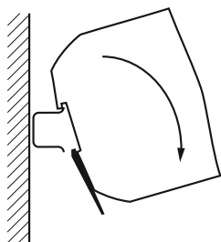
Fig. 15a Snap-fit mounting to DIN-Rail.
