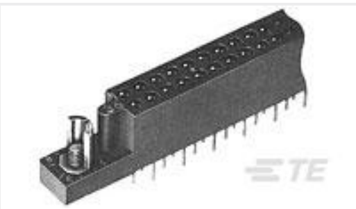
TE Part #1-530776-3 2 ROW BOX RECP 140 POS STAG
