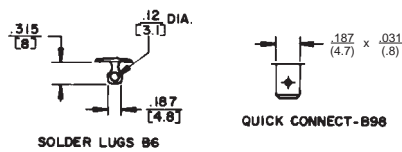
SOLDER LUGS -86
