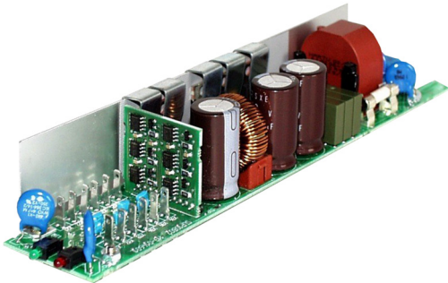
Application: DC/DC converter for supply power to fans (with monitoring)
