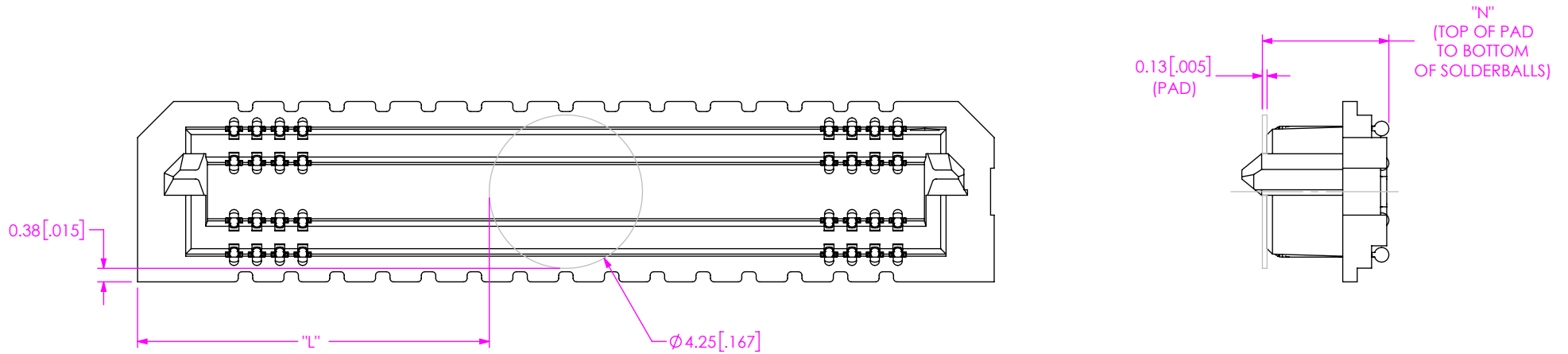
FIG 2 POLYIMIDE PAD ADM6-30-1.5-XXX-4-X-XR SHOWN (SAME AS FIG1, EXCEPT AS SHOWN) (SOME CENTER FEATURES REMOVED FOR CLARITY)
