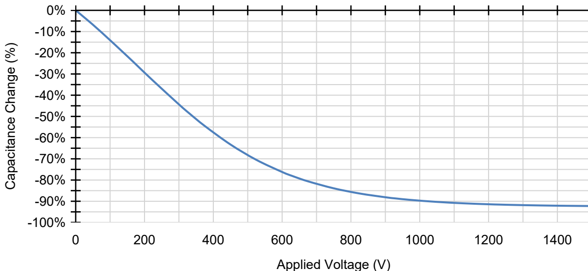
VCC Characterization
