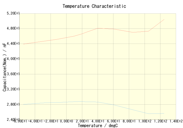
C3216X7R2E473K160AA(DC Bias = 0V) C3216X7R2E473K160AA(DC Bias = 125V)
