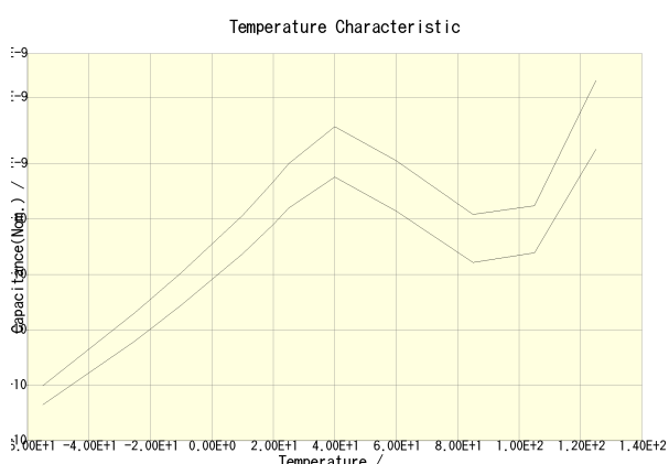
CKCL22X7R1H102M085AA(DC Bias = 0V) CKCL22X7R1H102M085AA(DC Bias = 25V)
