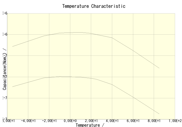
C2012X5R1C105K085AA(DC Bias = 0V) C2012X5R1C105K085AA(DC Bias = 8V)
