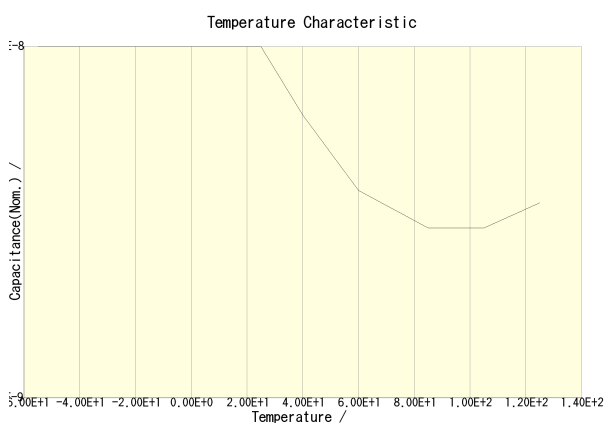
C3216C0G2A103J115AA(DC Bias = 0V) C3216C0G2A103J115AA(DC Bias = 50V)
