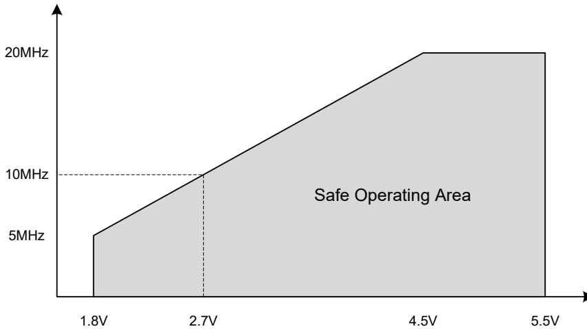
Figure 33-1. Maximum Frequency vs. V_{DD} for [-40, 105]^{\circ}\text{C}
