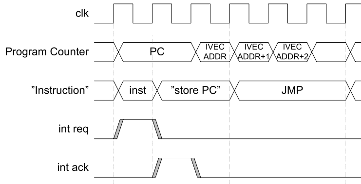
Figure 13-2. Interrupt Execution of a Single Cycle Instruction, Multicycle Instruction and from Sleep Single Cycle Instruction
