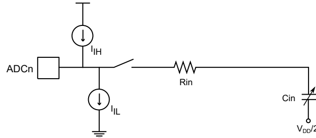
Figure 30-11. Analog Input Schematic
