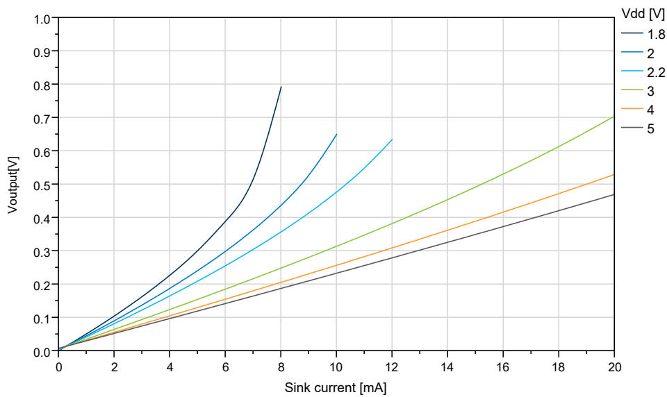
Figure 34-24. : IO Pin Output Voltage vs. Sink Current ( T=25^{\circ}C )
