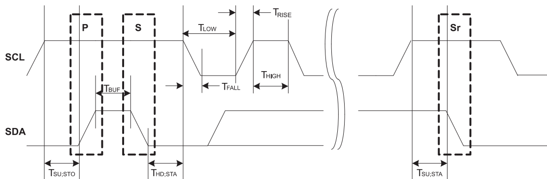
Figure 26-14. SCL Timing
